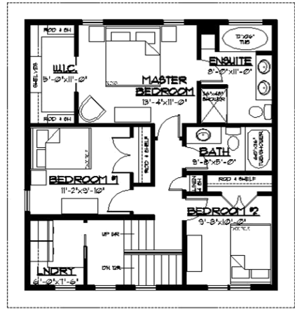
SECOND FLOOR PLAN OPTION #1
