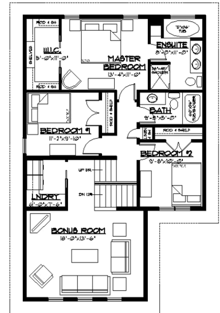
SECOND FLOOR PLAN OPTION #2
