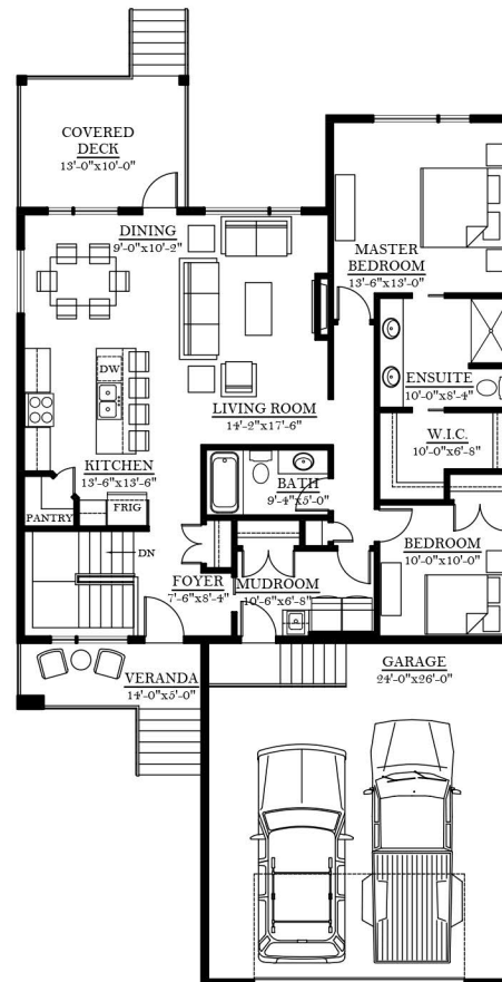
MAIN FLOOR PLAN AREA: 1356 SQ FT
