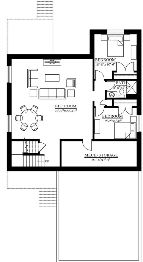
BASEMENT PLAN AREA: 1356 SQ FT
