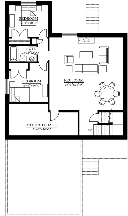
BASEMENT PLAN AREA: 1399 SQ FT
