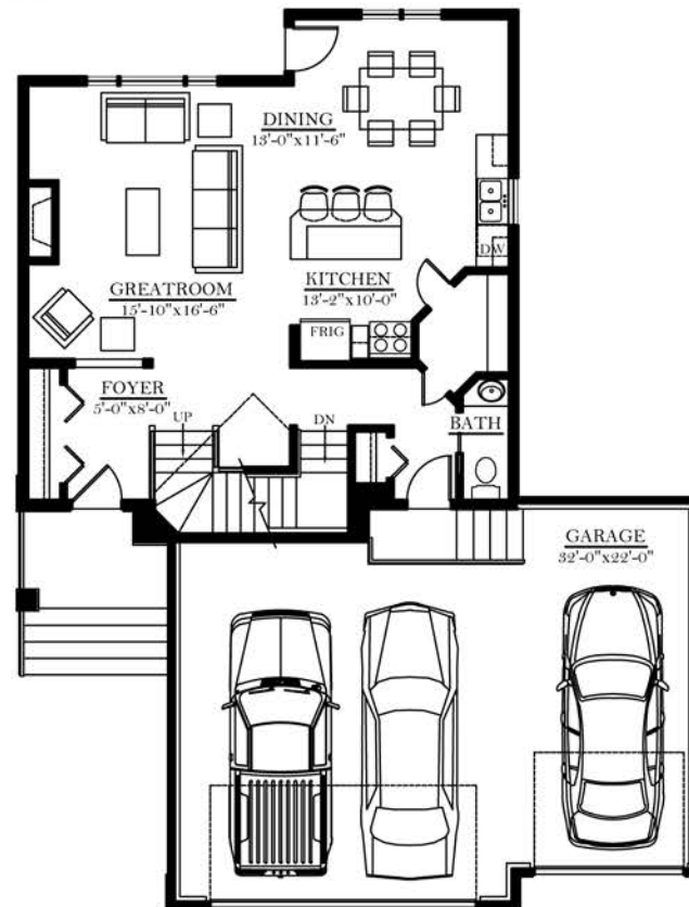
MAIN FLOOR PLAN 836 SQ. FT.
