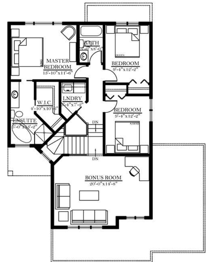
SECOND FLOOR PLAN 1114 SQ. FT.
